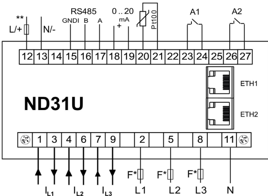
Fig. 4. Meter connections
